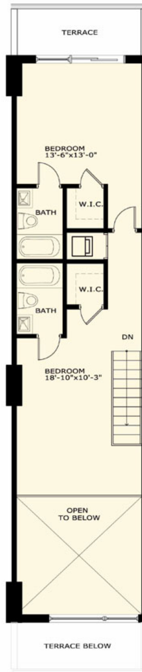
SECOND FLOOR
