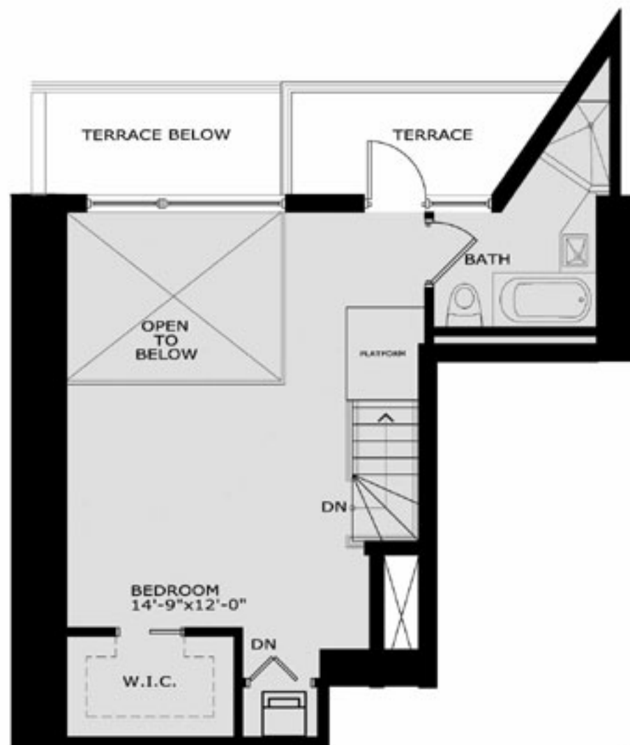
SECOND FLOOR
